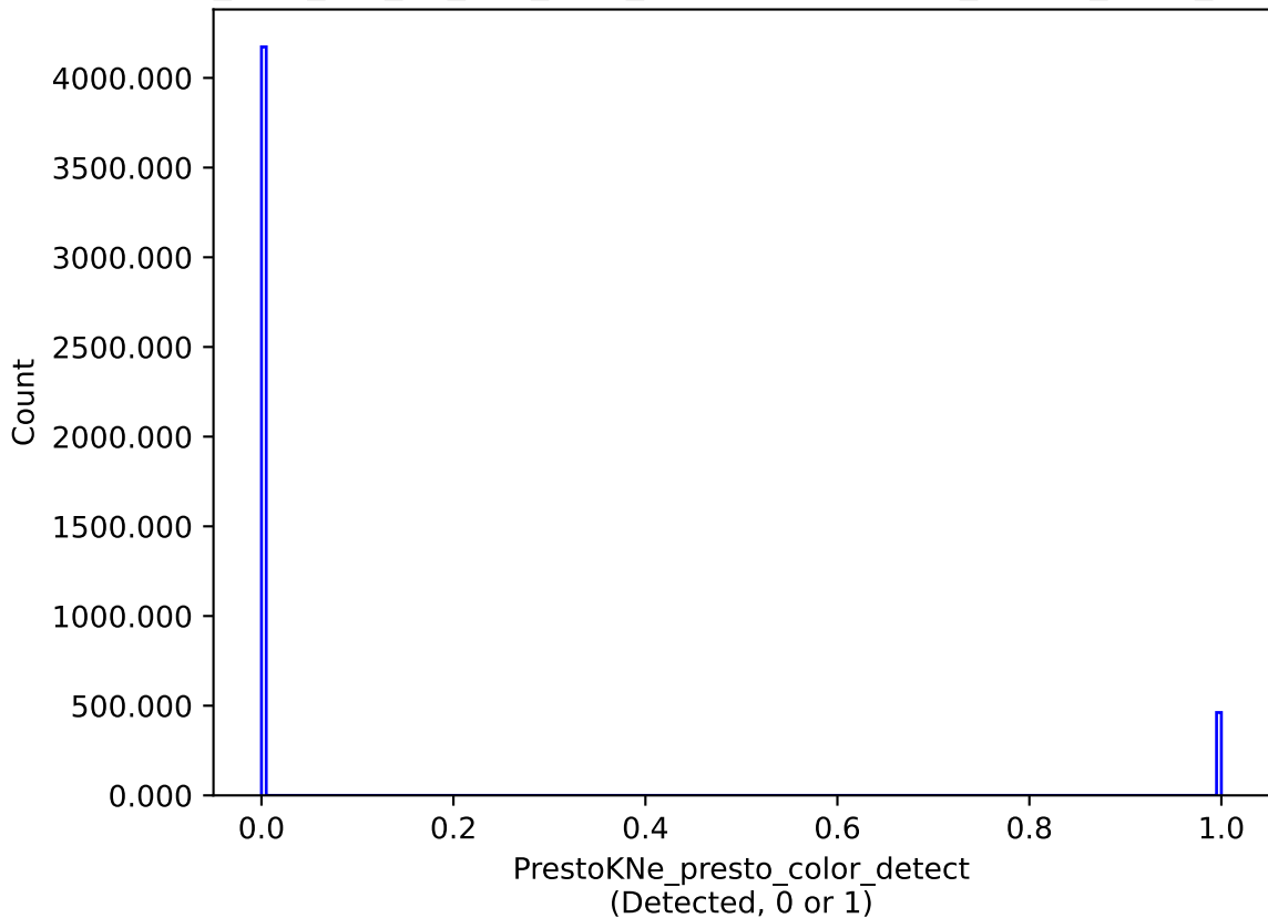
too_elab_r16_d2_griz_v3.4_10yrs : PrestoKNe_presto_color_detect
