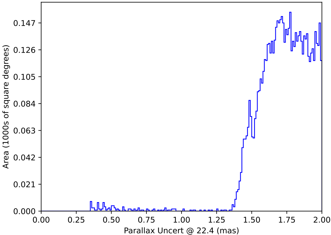
too_elab_r16_d2_griz_v3.4_10yrs : Parallax Uncert @ 22.4
