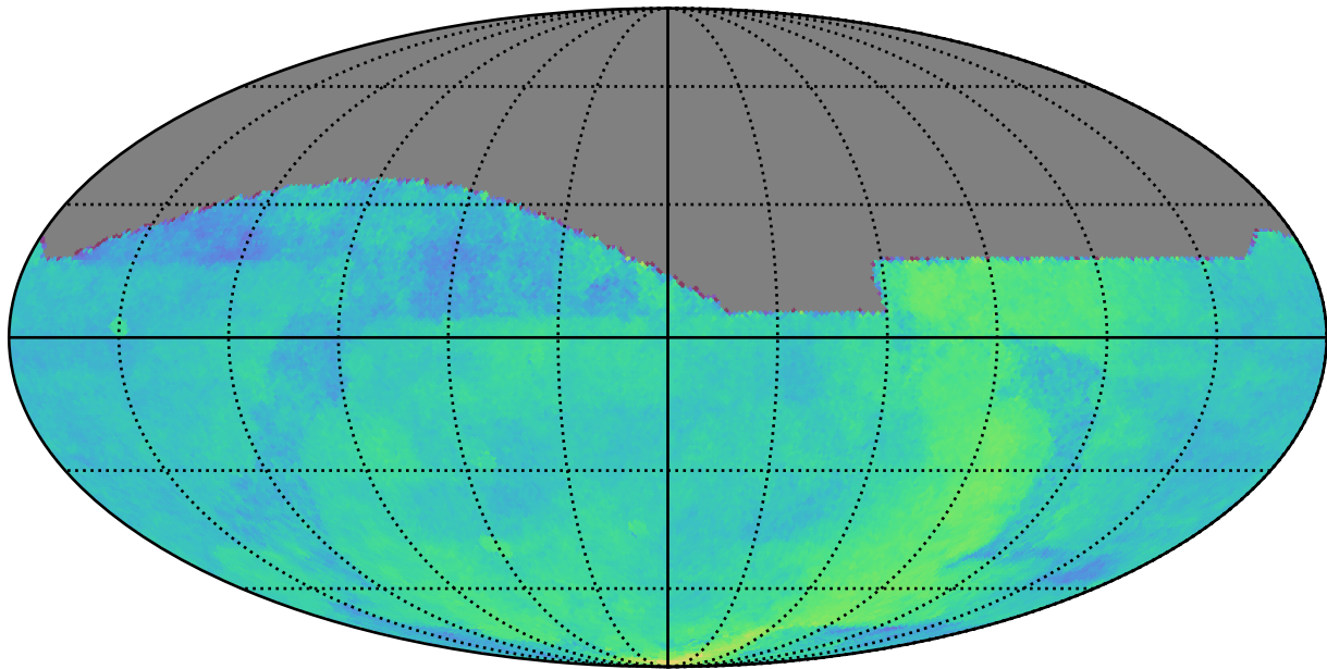
too_elab_r16_d2_griz_v3.4_10yrs : Parallax Coverage @ 22.4
