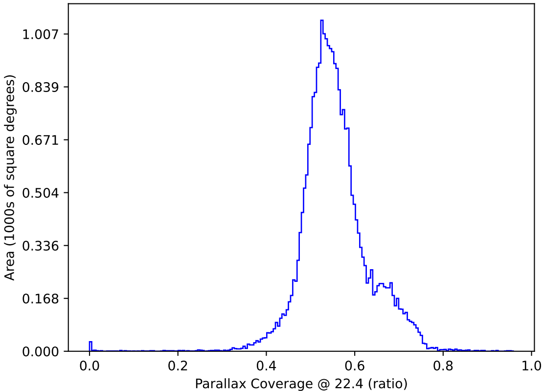
too_elab_r16_d2_griz_v3.4_10yrs : Parallax Coverage @ 22.4
