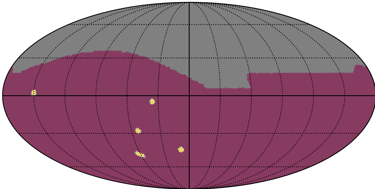
too_elab_r16_d2_griz_v3.4_10yrs : NumberOfQuickRevisits
