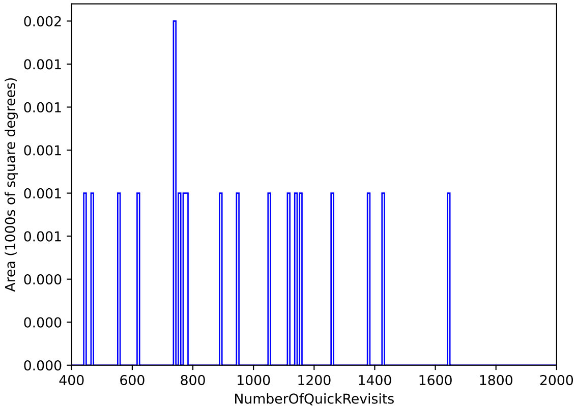
too_elab_r16_d2_griz_v3.4_10yrs : NumberOfQuickRevisits
