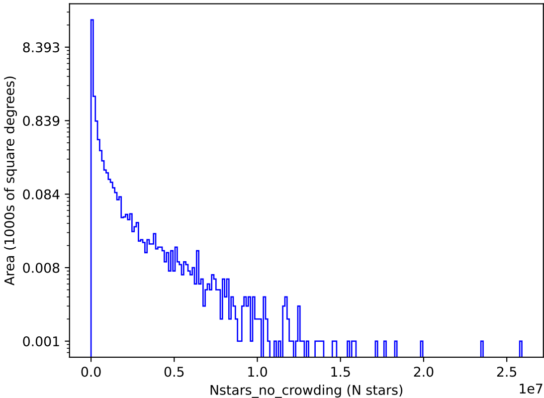
too_elab_r16_d2_griz_v3.4_10yrs y: Nstars_no_crowding
