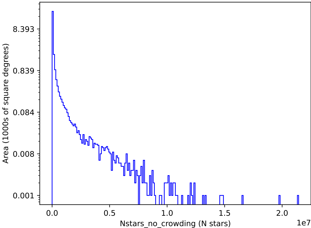
too_elab_r16_d2_griz_v3.4_10yrs r: Nstars_no_crowding
