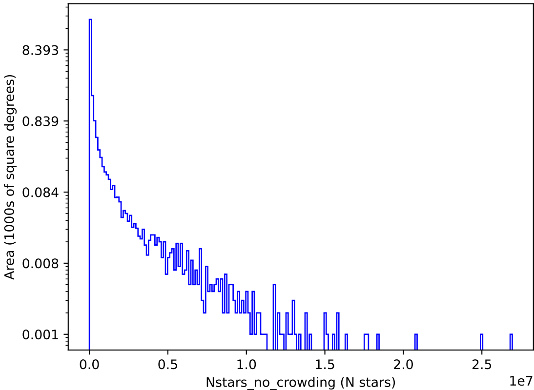
too_elab_r16_d2_griz_v3.4_10yrs i: Nstars_no_crowding
