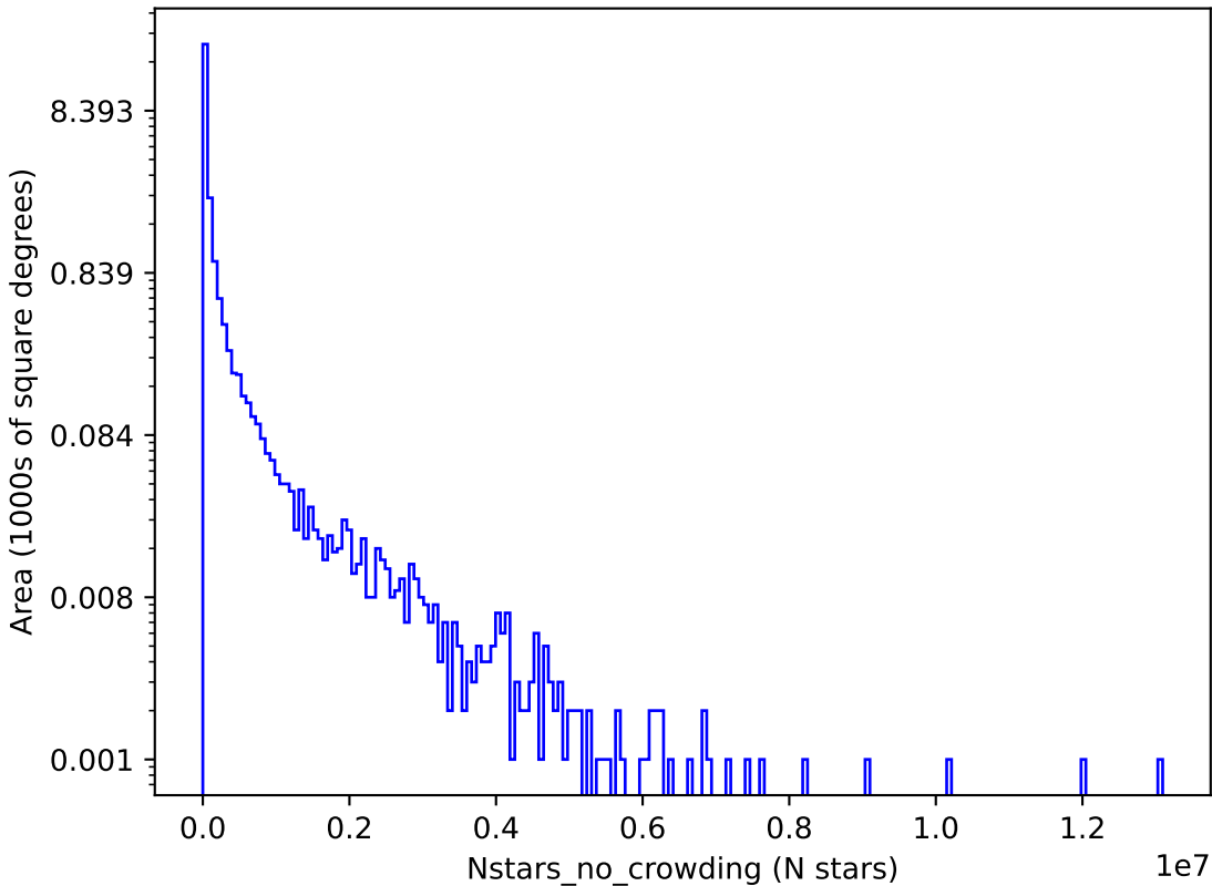
too_elab_r16_d2_griz_v3.4_10yrs g: Nstars_no_crowding
