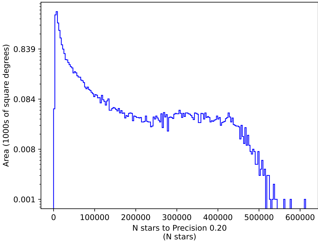
too_elab_r16_d2_griz_v3.4_10yrs g: N stars to Precision 0.20
