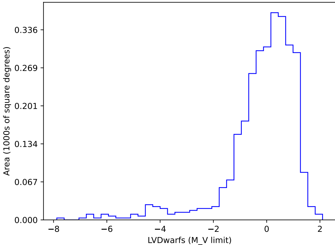
too_elab_r16_d2_griz_v3.4_10yrs gi SCP: LVDwarfs
