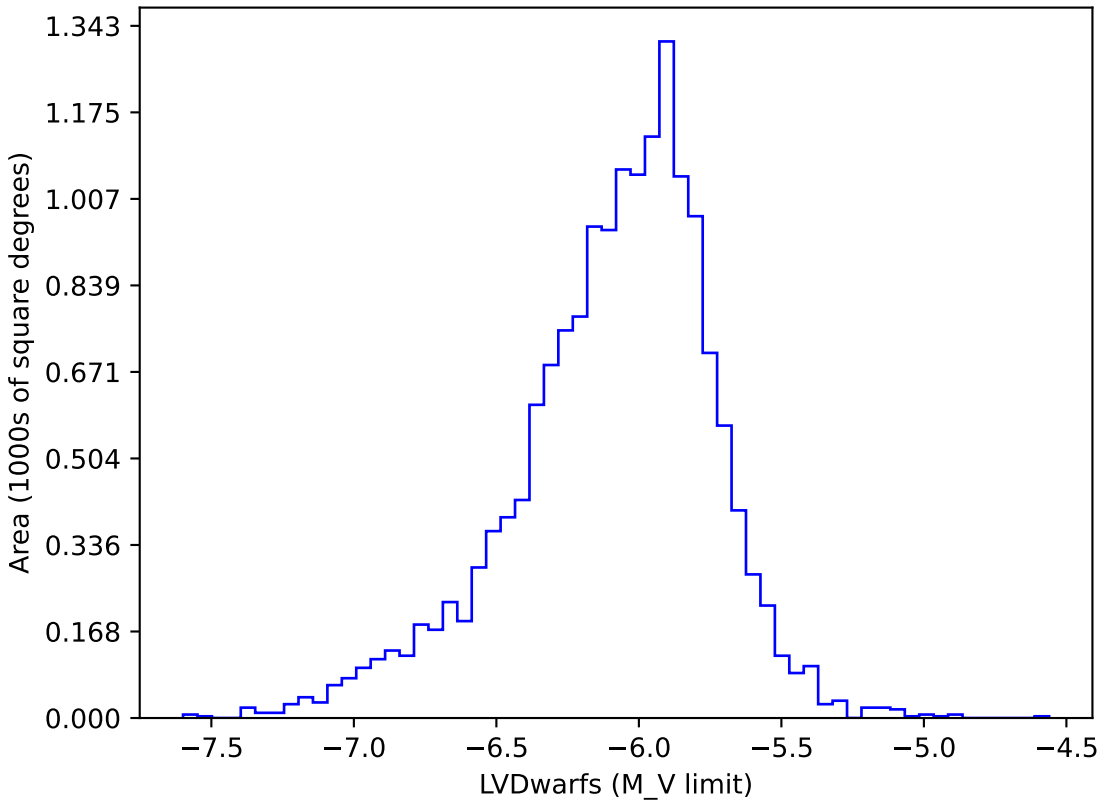
too_elab_r16_d2_griz_v3.4_10yrs gi: LVDwarfs
