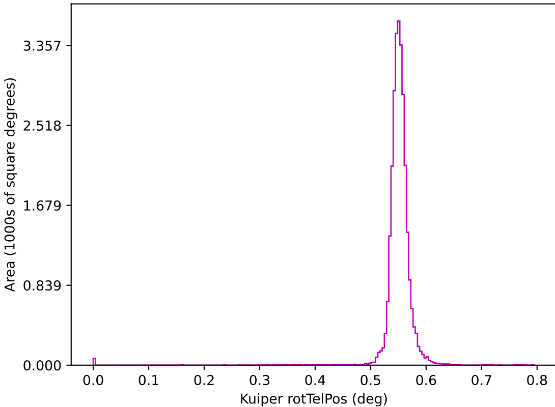
too_elab_r16_d2_griz_v3.4_10yrs z: Kuiper rotTelPos
