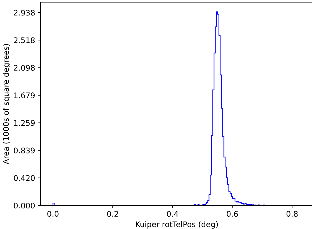
too_elab_r16_d2_griz_v3.4_10yrs y: Kuiper rotTelPos
