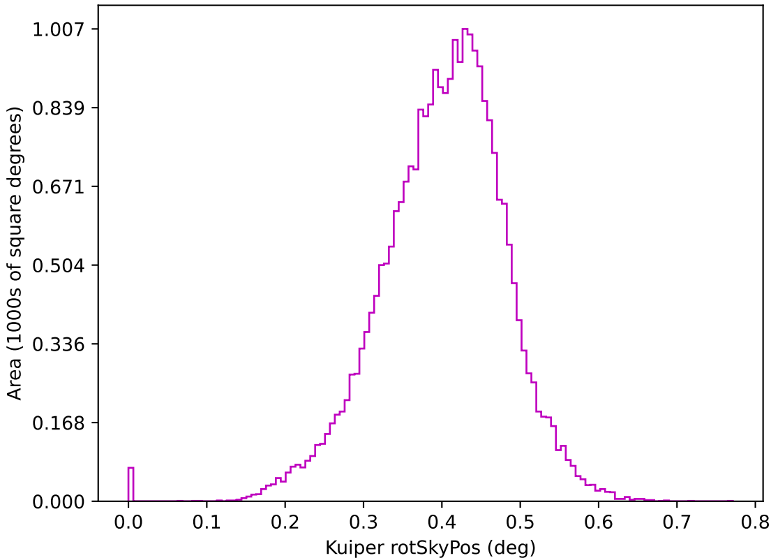
too_elab_r16_d2_griz_v3.4_10yrs z: Kuiper rotSkyPos
