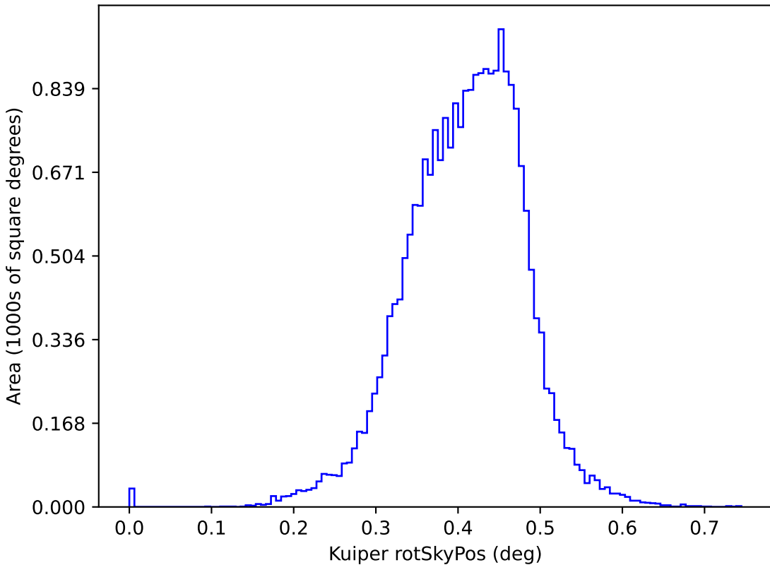
too_elab_r16_d2_griz_v3.4_10yrs y: Kuiper rotSkyPos
