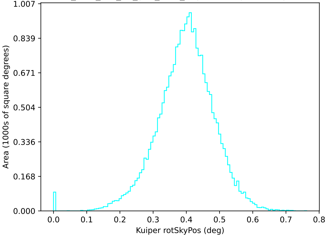
too_elab_r16_d2_griz_v3.4_10yrs u: Kuiper rotSkyPos
