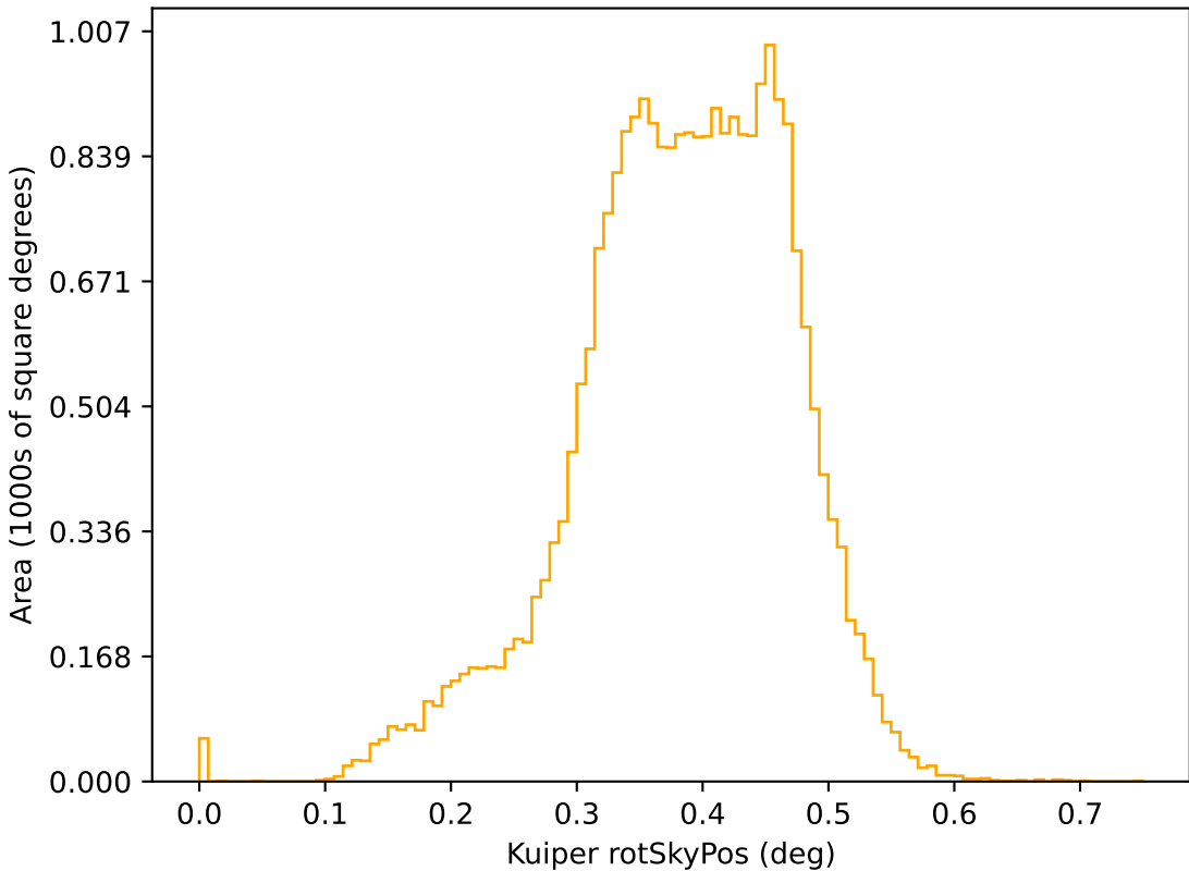
too_elab_r16_d2_griz_v3.4_10yrs r: Kuiper rotSkyPos
