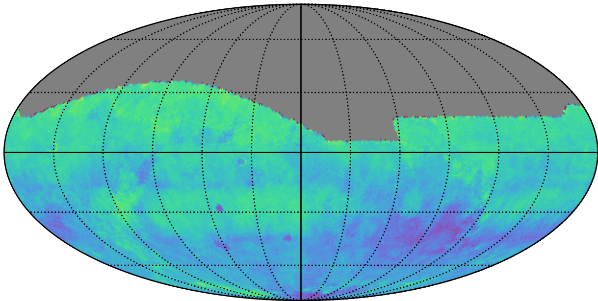
too_elab_r16_d2_griz_v3.4_10yrs i: Kuiper rotSkyPos
