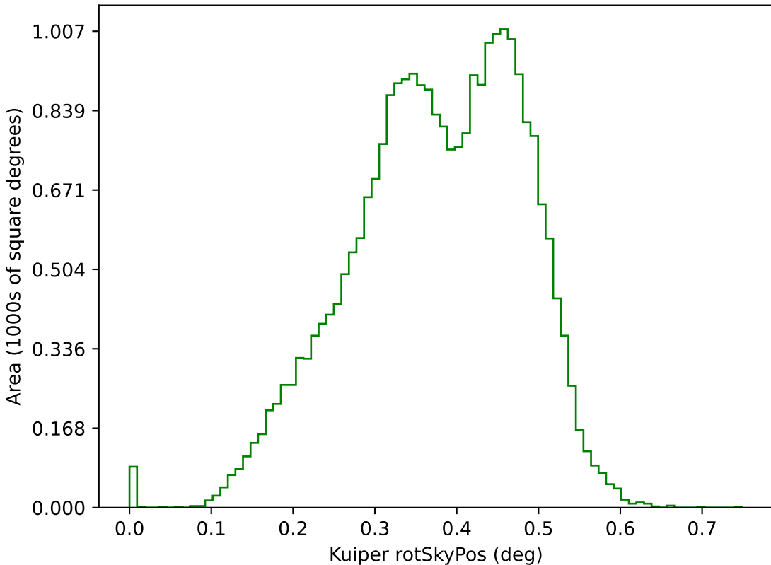
too_elab_r16_d2_griz_v3.4_10yrs g: Kuiper rotSkyPos
