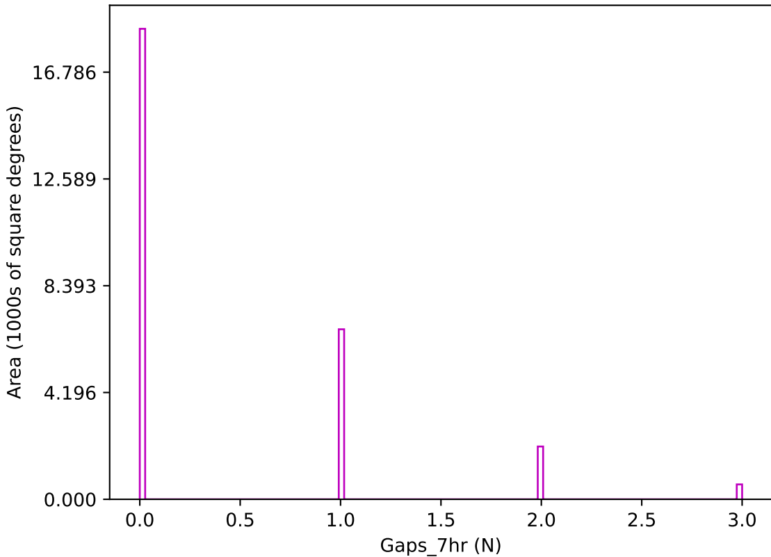
too_elab_r16_d2_griz_v3.4_10yrs z band: Gaps_7hr
