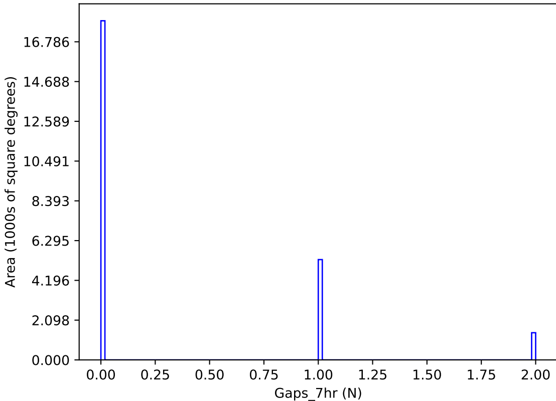
too_elab_r16_d2_griz_v3.4_10yrs y band: Gaps_7hr
