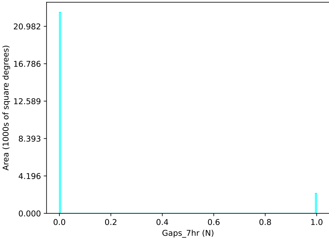
too_elab_r16_d2_griz_v3.4_10yrs u band: Gaps_7hr
