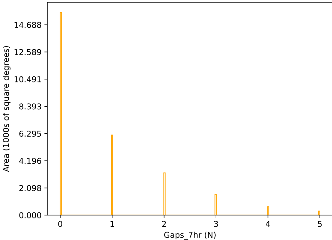
too_elab_r16_d2_griz_v3.4_10yrs r band: Gaps_7hr
