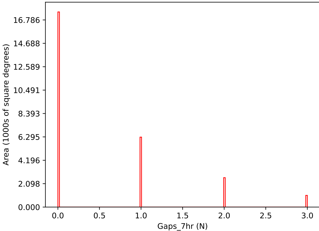
too_elab_r16_d2_griz_v3.4_10yrs i band: Gaps_7hr
