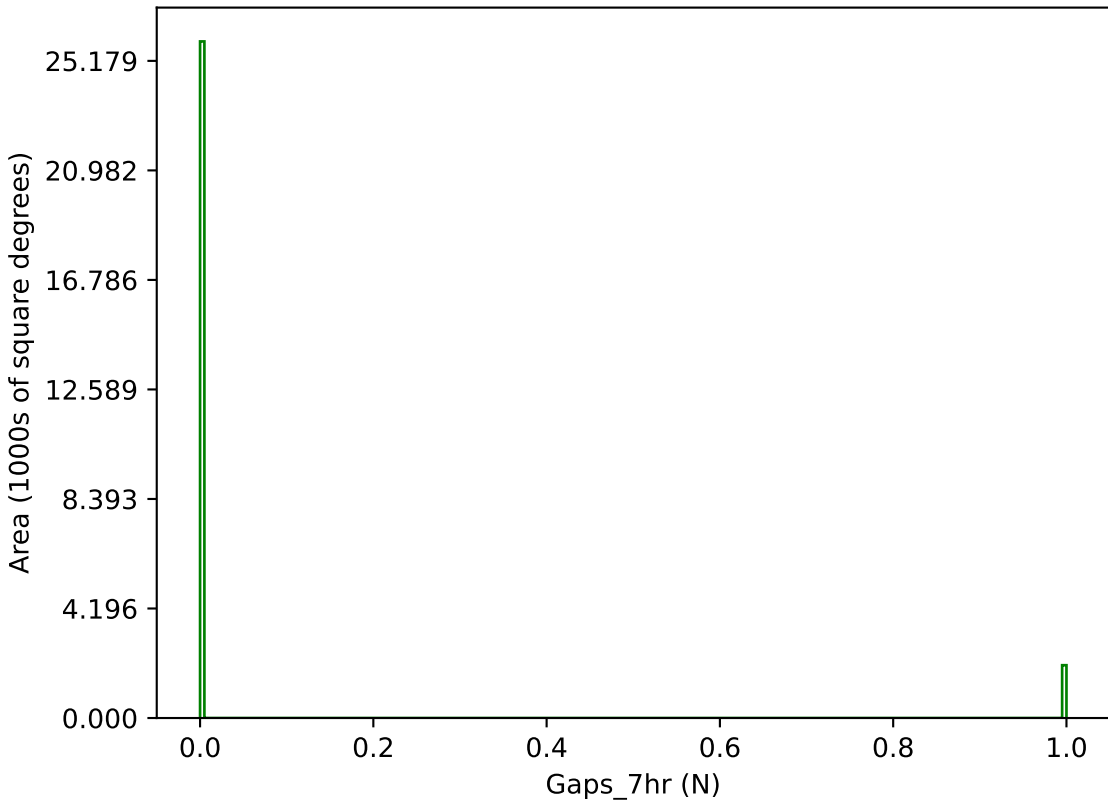
too_elab_r16_d2_griz_v3.4_10yrs g band: Gaps_7hr
