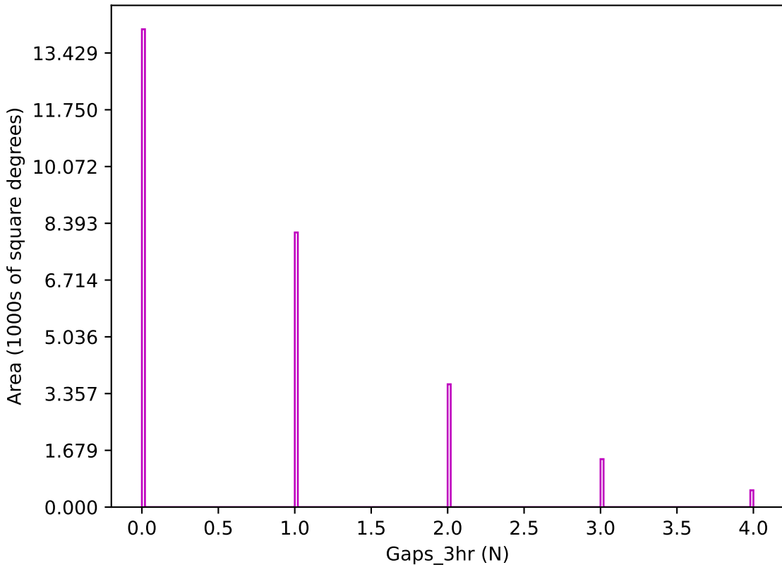
too_elab_r16_d2_griz_v3.4_10yrs z band: Gaps_3hr
