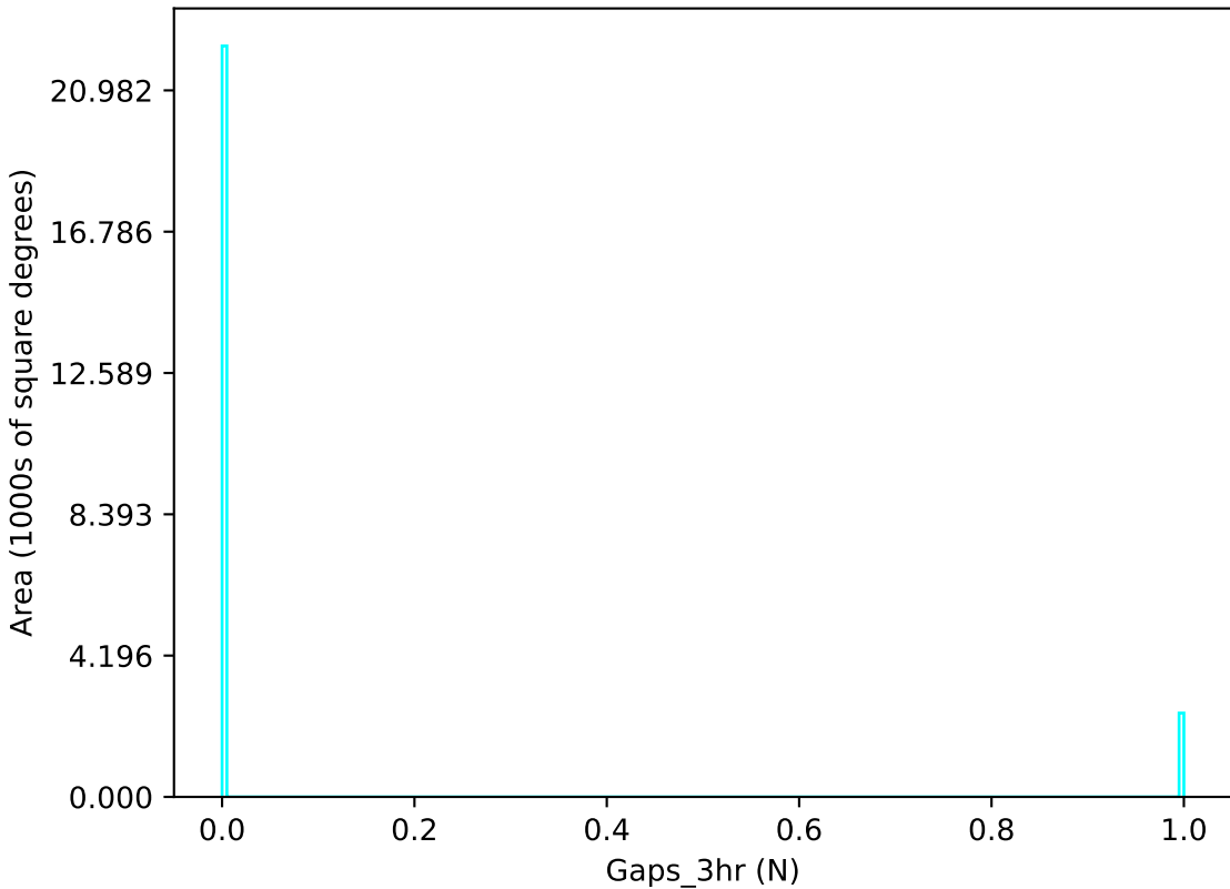
too_elab_r16_d2_griz_v3.4_10yrs u band: Gaps_3hr
