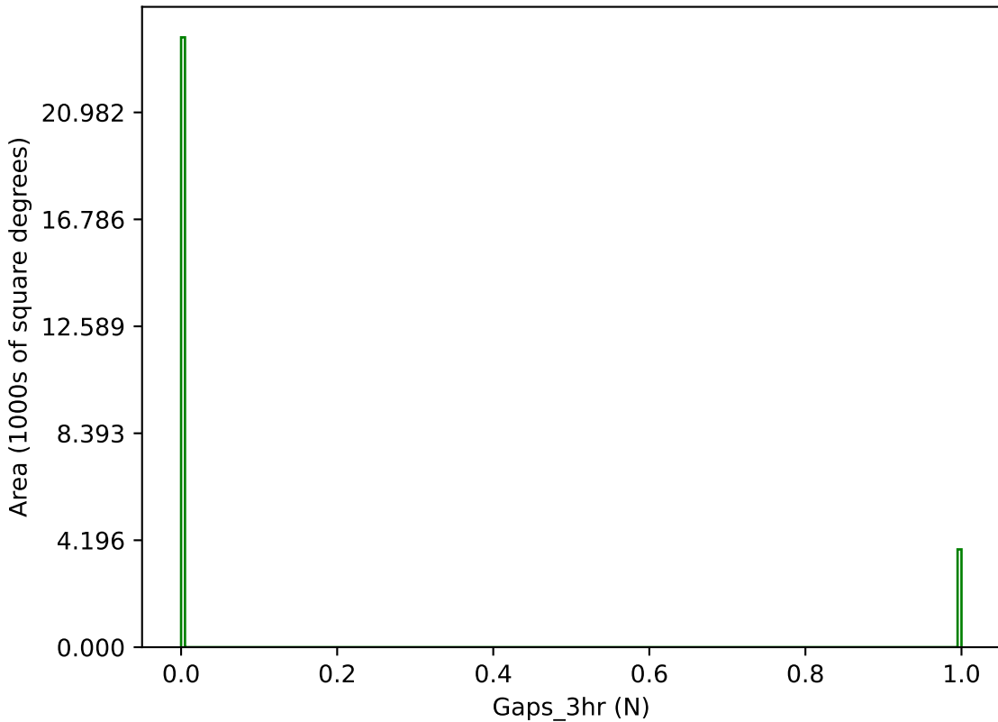
too_elab_r16_d2_griz_v3.4_10yrs g band: Gaps_3hr
