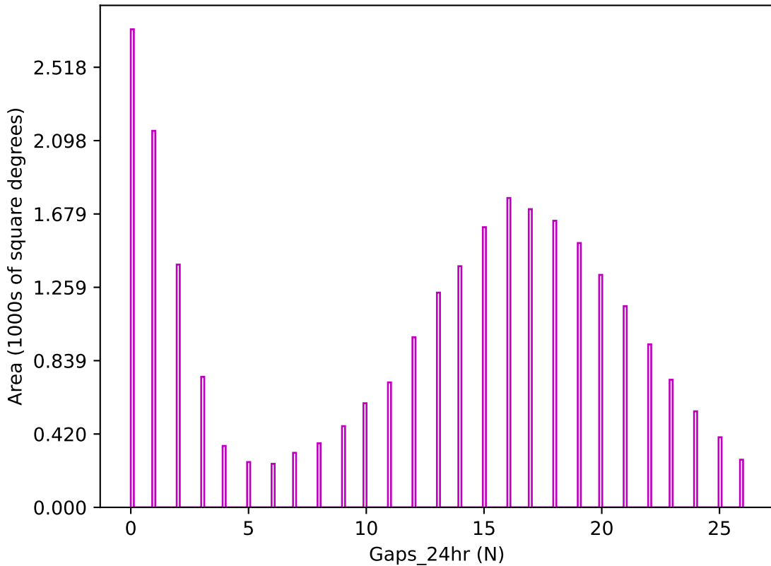
too_elab_r16_d2_griz_v3.4_10yrs z band: Gaps_24hr
