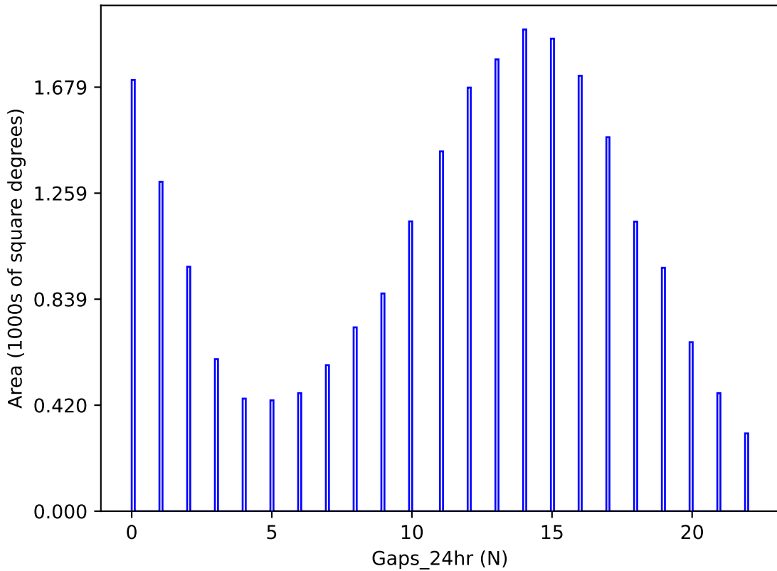
too_elab_r16_d2_griz_v3.4_10yrs y band: Gaps_24hr
