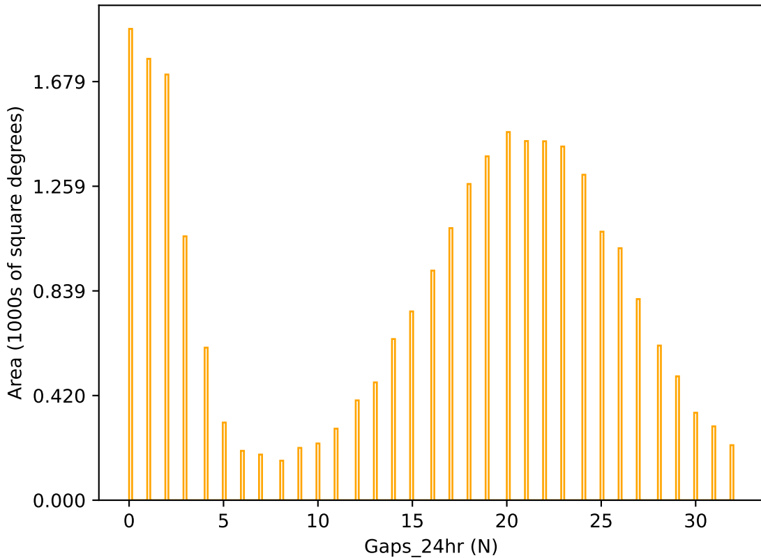
too_elab_r16_d2_griz_v3.4_10yrs r band: Gaps_24hr
