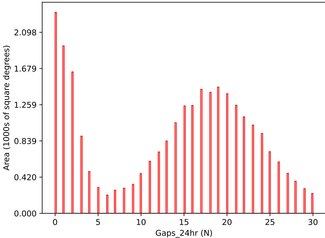
too_elab_r16_d2_griz_v3.4_10yrs i band: Gaps_24hr
