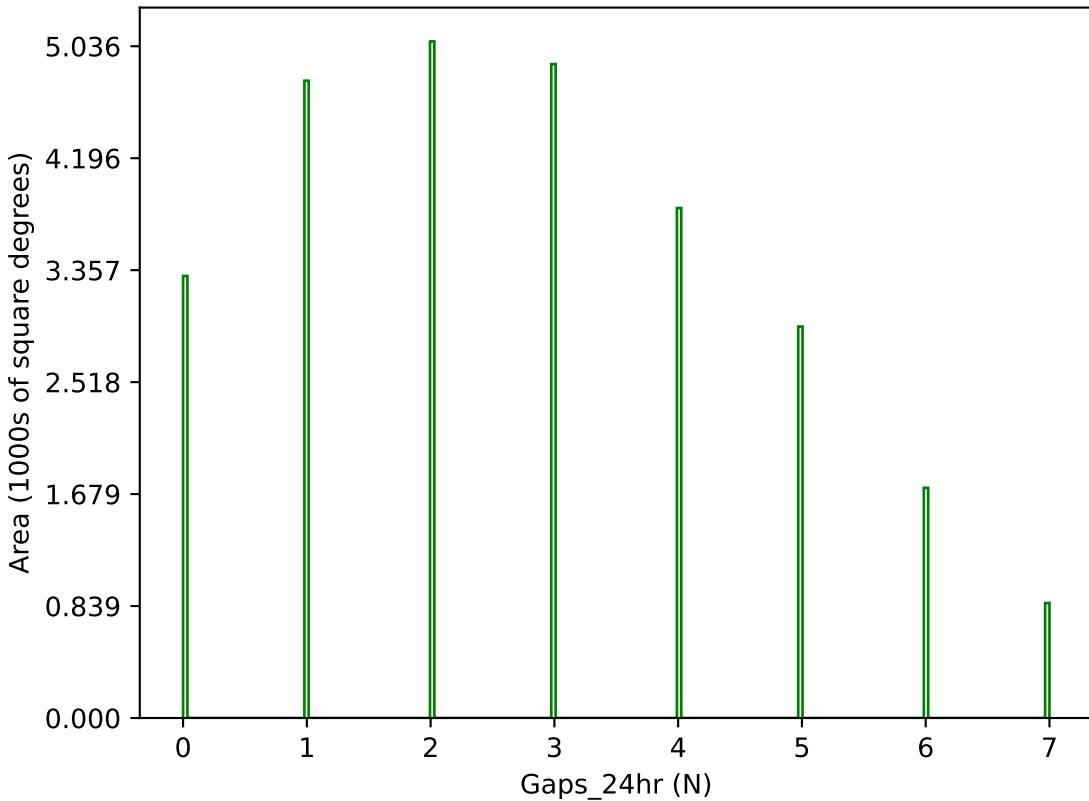
too_elab_r16_d2_griz_v3.4_10yrs g band: Gaps_24hr
