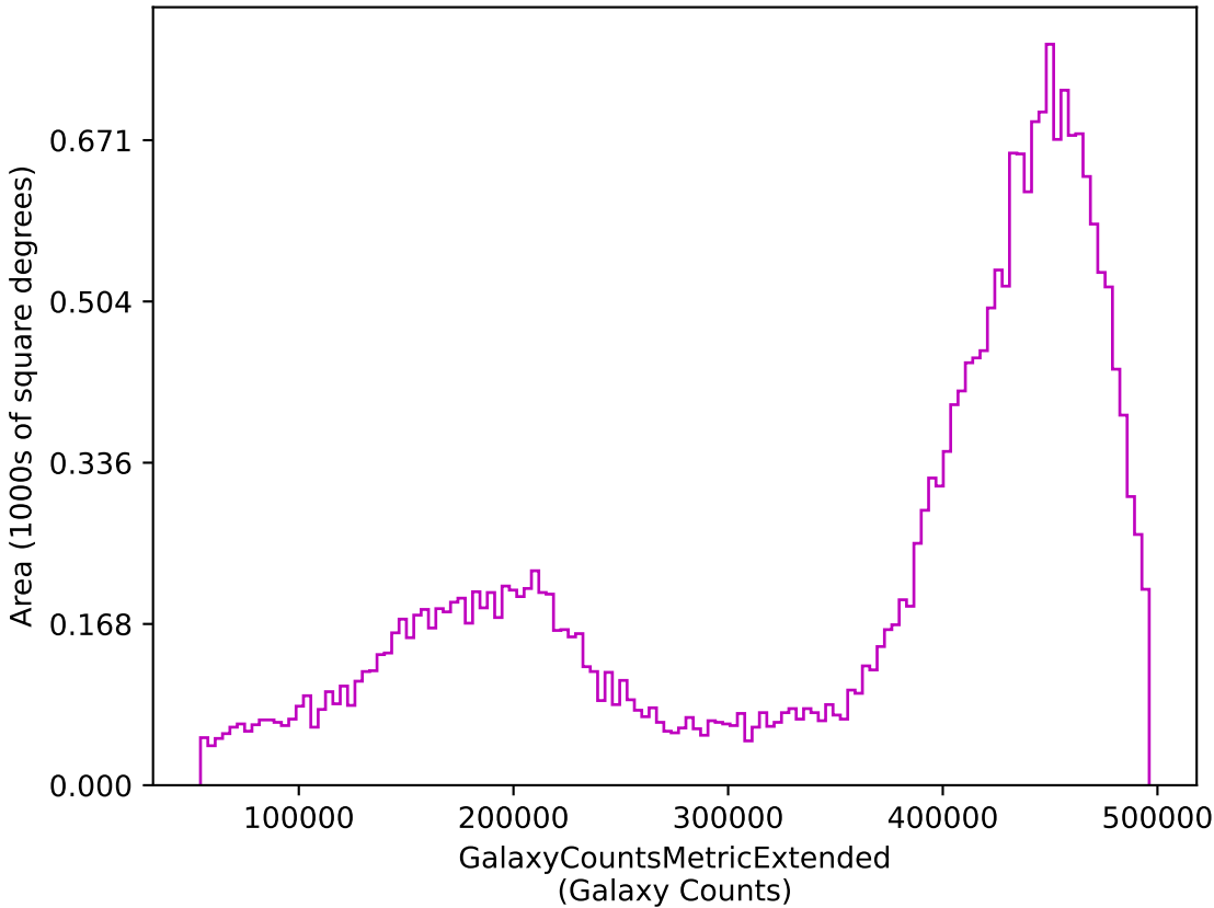
too_elab_r16_d2_griz_v3.4_10yrs z: GalaxyCountsMetricExtended
