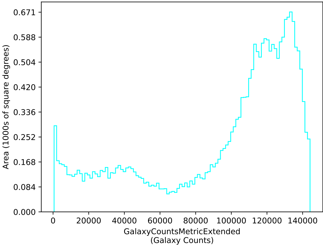
too_elab_r16_d2_griz_v3.4_10yrs u: GalaxyCountsMetricExtended
