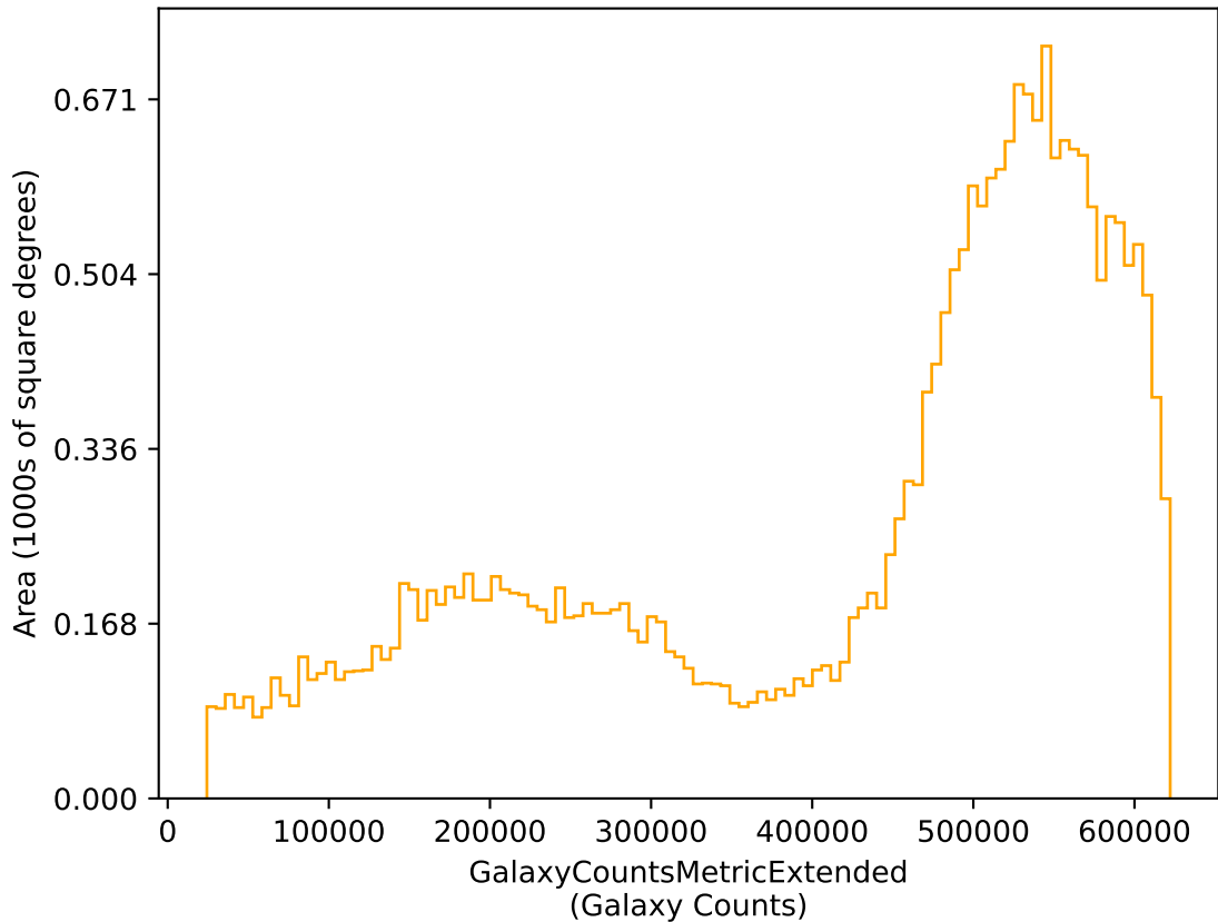
too_elab_r16_d2_griz_v3.4_10yrs r: GalaxyCountsMetricExtended
