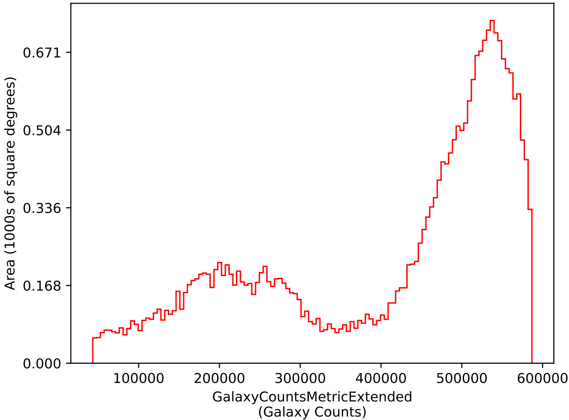
too_elab_r16_d2_griz_v3.4_10yrs i: GalaxyCountsMetricExtended
