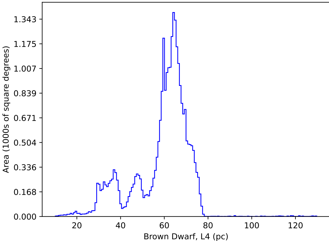
too_elab_r16_d2_griz_v3.4_10yrs : Brown Dwarf, L4
