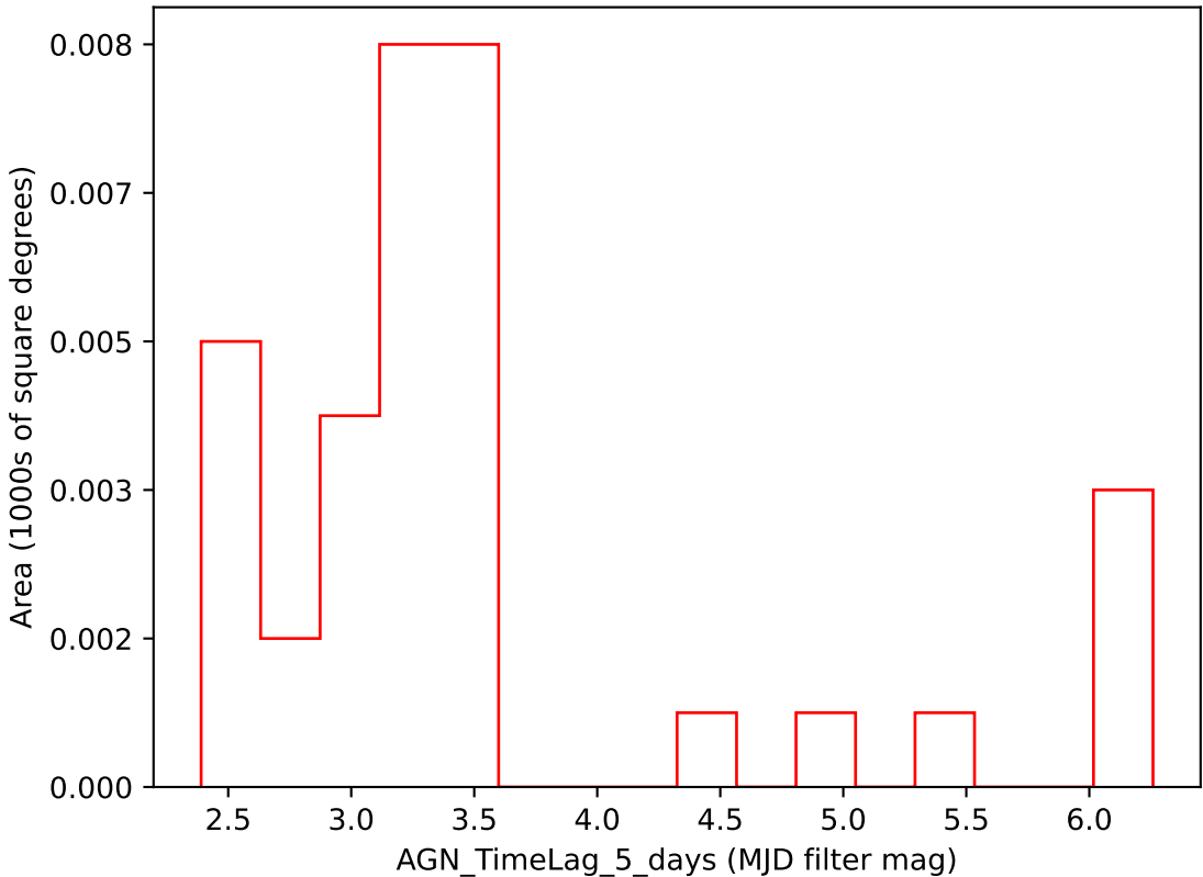
too_elab_r16_d2_griz_v3.4_10yrs i band: AGN_TimeLag_5_days
