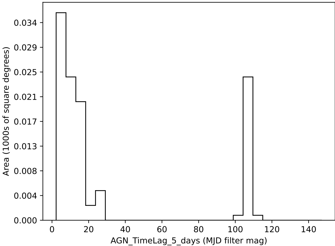
too_elab_r16_d2_griz_v3.4_10yrs all bands: AGN_TimeLag_5_days
