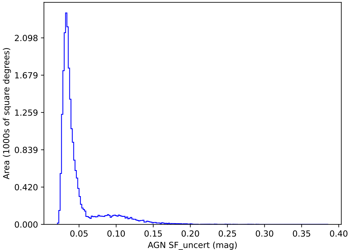
too_elab_r16_d2_griz_v3.4_10yrs y band: AGN SF_uncert
