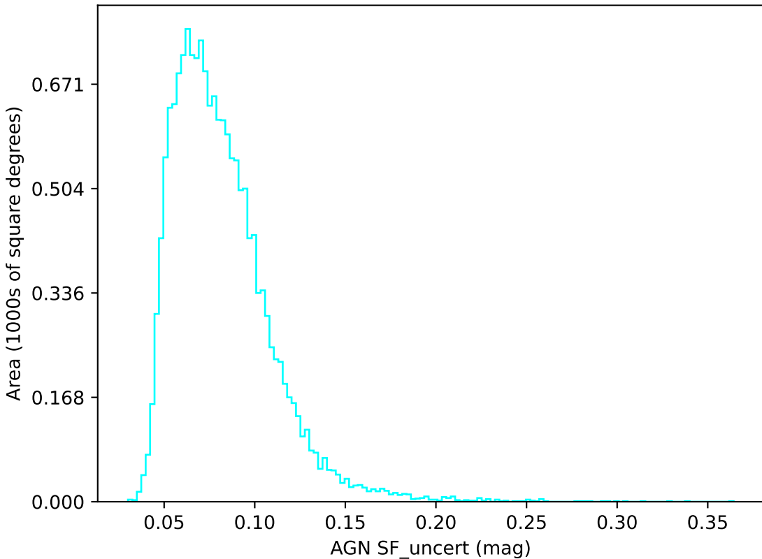
too_elab_r16_d2_griz_v3.4_10yrs u band: AGN SF_uncert
