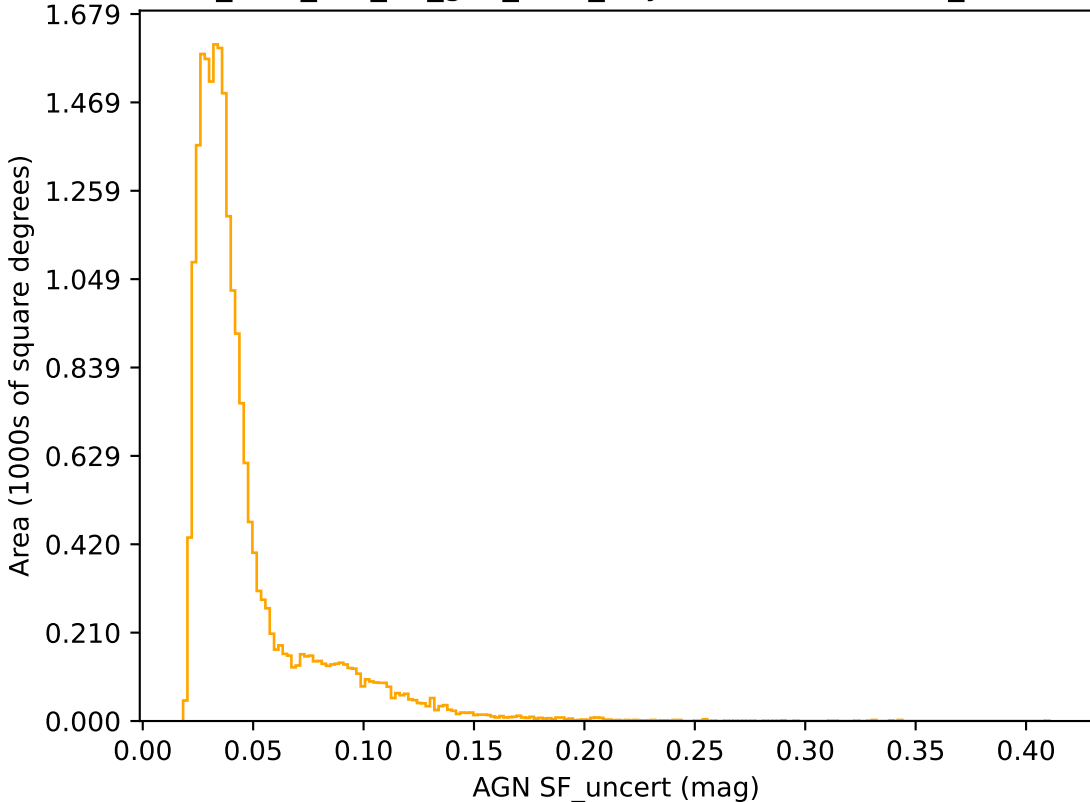
too_elab_r16_d2_griz_v3.4_10yrs r band: AGN SF_uncert
