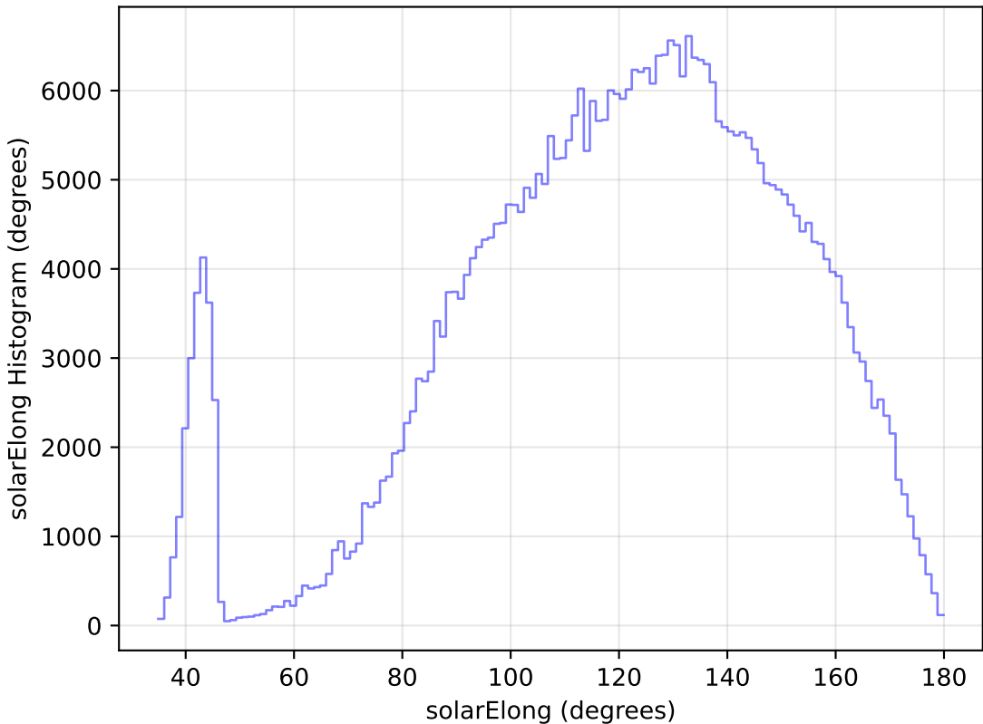
too_elab_r16_d2_griz_v3.4_10yrs WFD z band: solarElong Histogram
