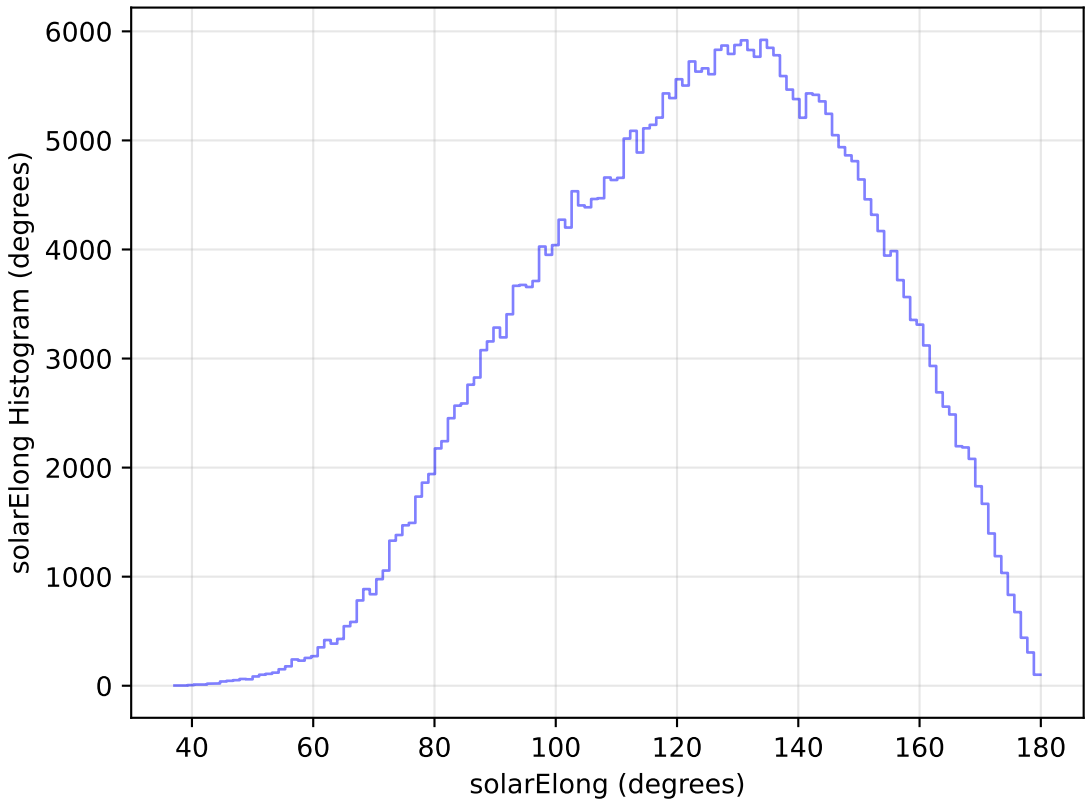
too_elab_r16_d2_griz_v3.4_10yrs WFD y band: solarElong Histogram
