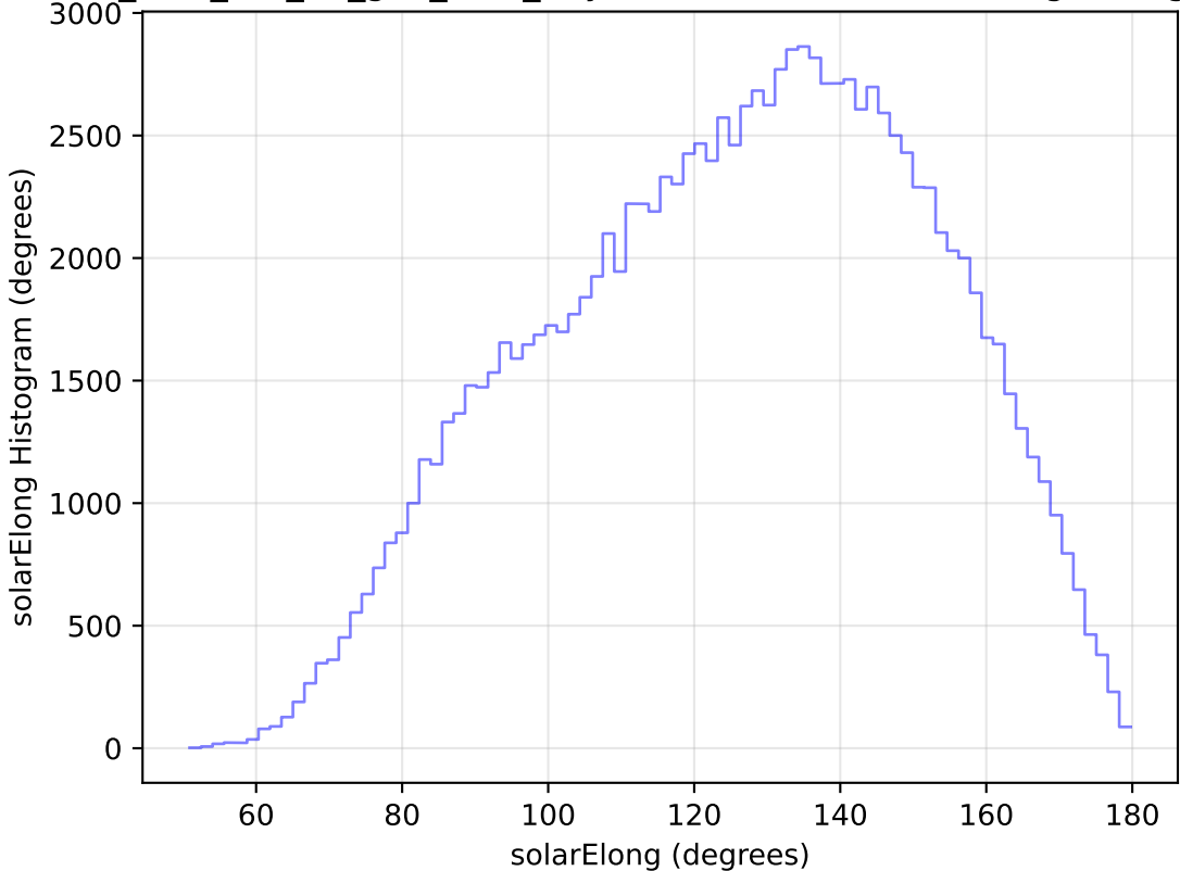
too_elab_r16_d2_griz_v3.4_10yrs WFD u band: solarElong Histogram
