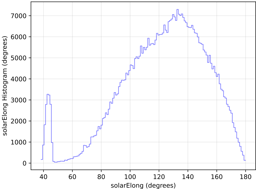
too_elab_r16_d2_griz_v3.4_10yrs WFD r band: solarElong Histogram
