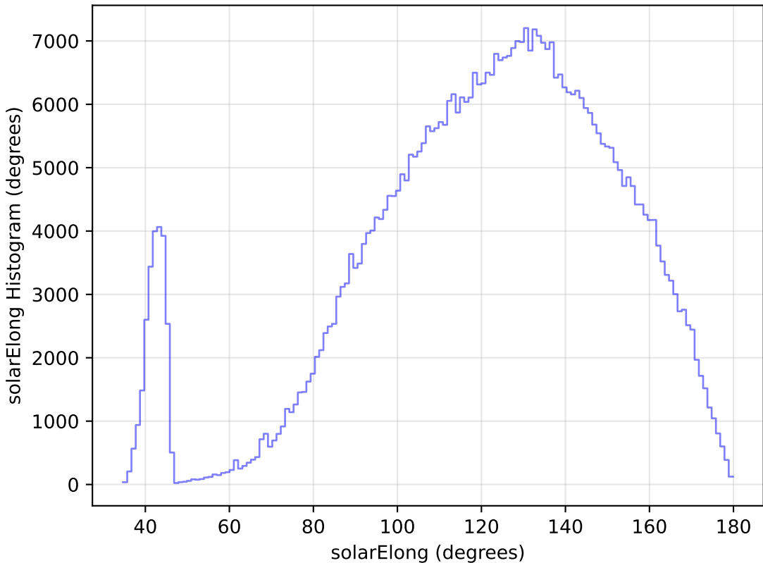
too_elab_r16_d2_griz_v3.4_10yrs WFD i band: solarElong Histogram
